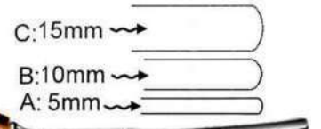
RIC-01-0556B Lexer Spongiosa Gouge (25 cm / 9 ¾")
